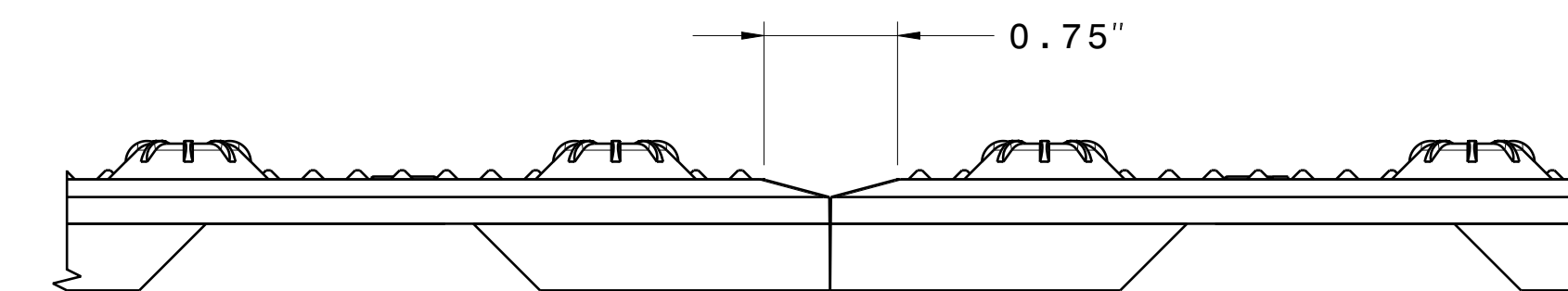
SIDE VIEW: 2-PANEL
