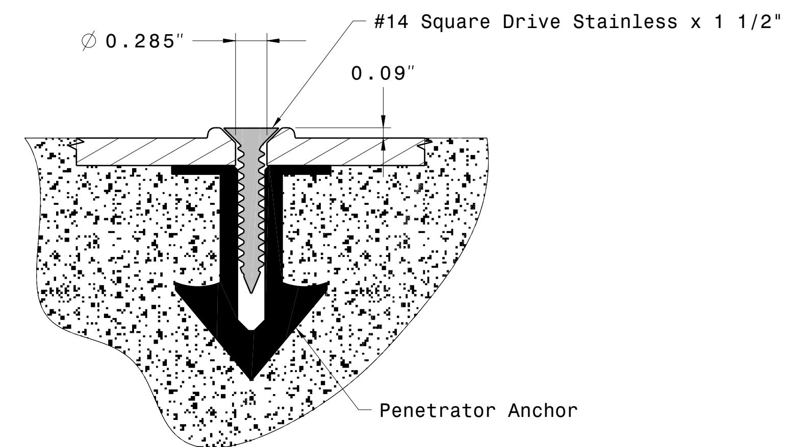
TYPICAL INTERIOR FASTENER DETAIL
