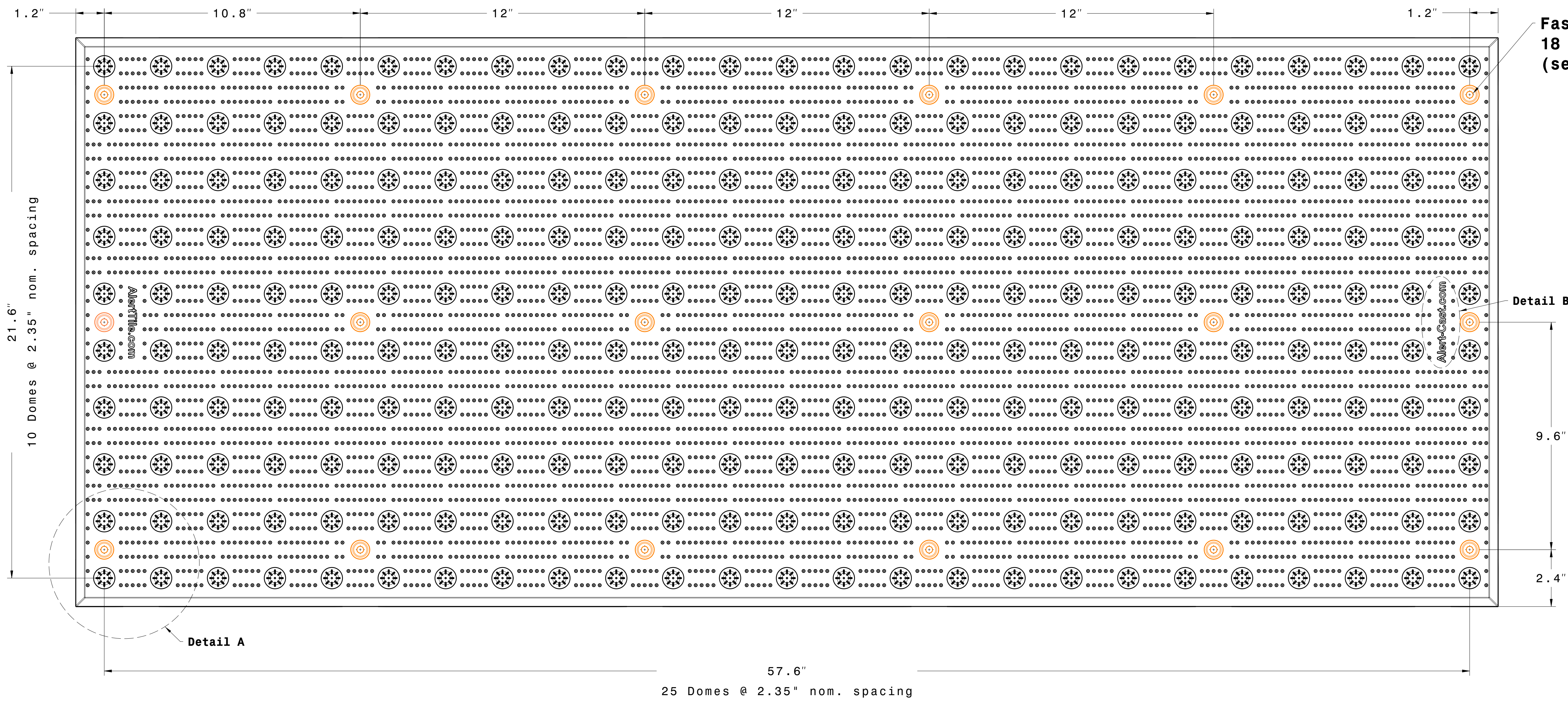
PLAN VIEW
