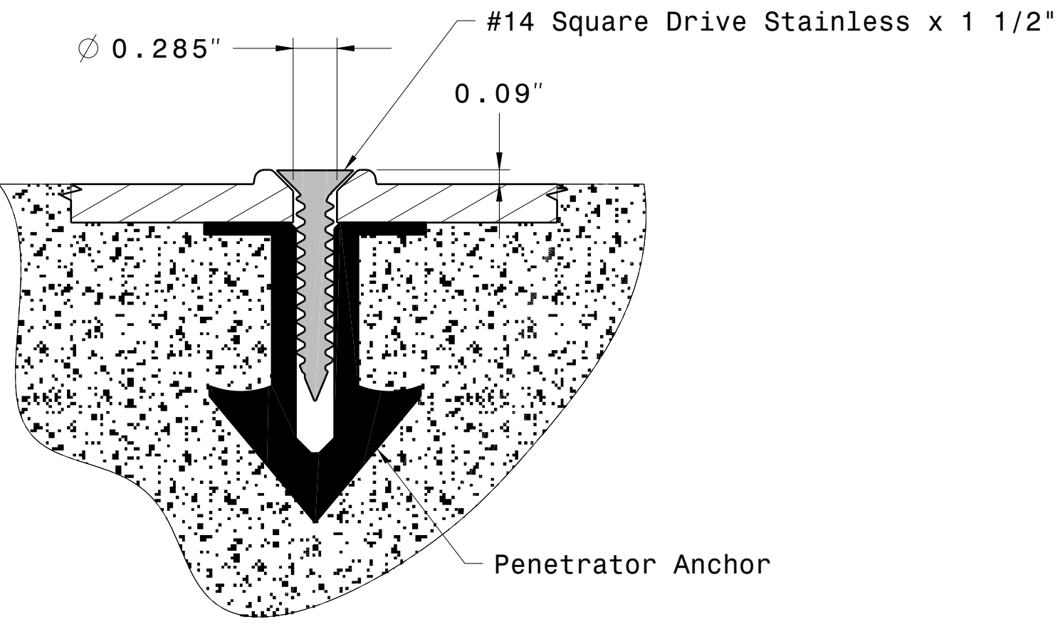
TYPICAL INTERIOR FASTENER DETAIL
