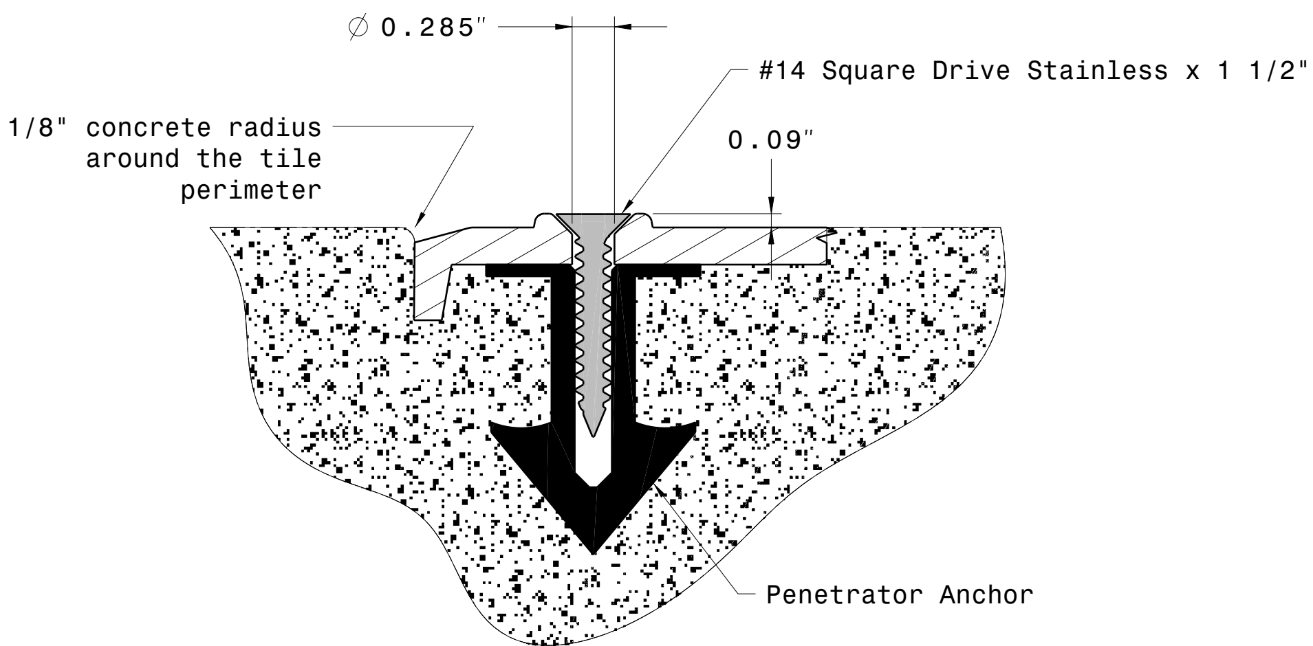
TYPICAL PERIMETER FASTENER DETAIL
