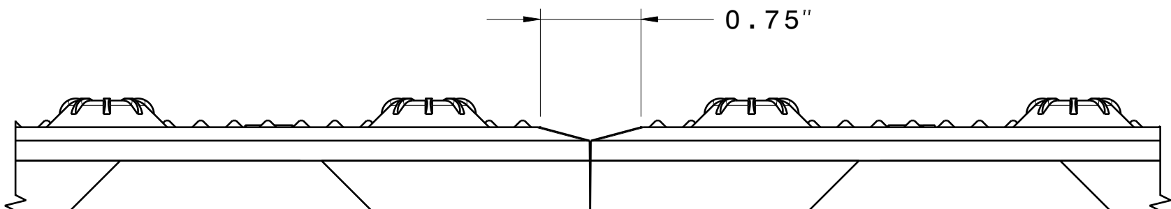
SIDE VIEW: 2-PANEL
