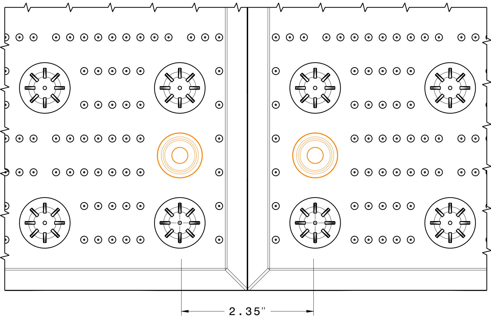
PLAN VIEW: 2-PANEL
