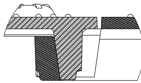
SECTION VIEW: INTERLOCKING FEATURE FOR ADJACENT PLATES
