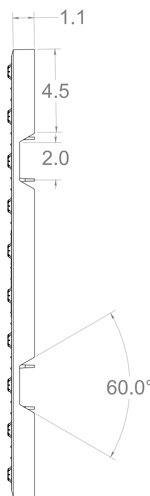
SIDE VIEW
