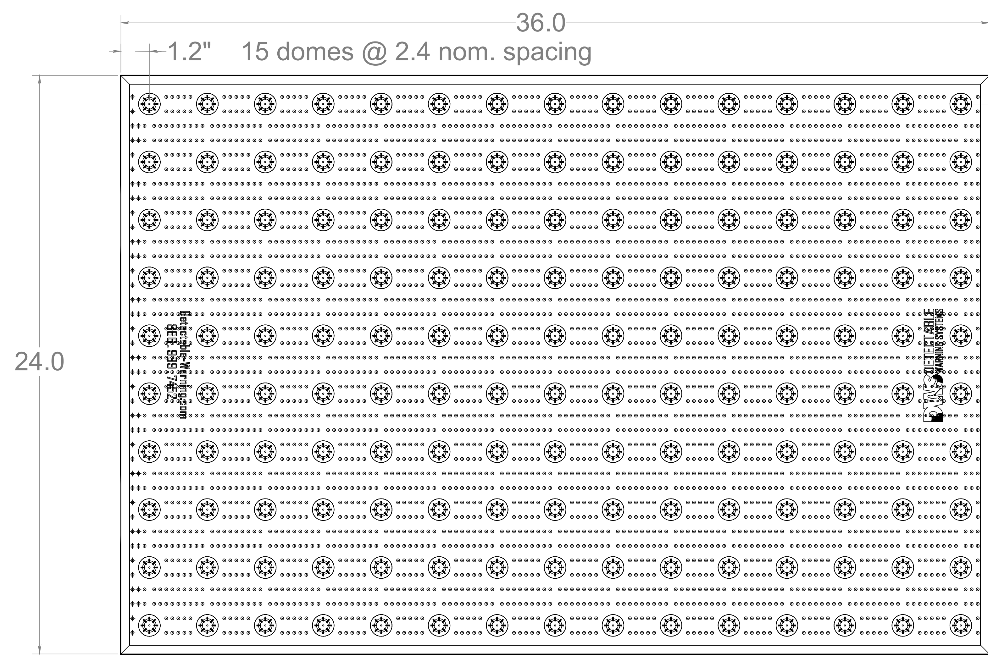
TOP VIEW
